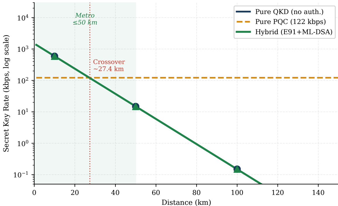
Fig. 5 — Secret Key Rate vs. Distance (p=0, asymptotic)
