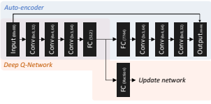
Fig. 4. Proposed network for Atari game: “Conv” means a convolutional layer.
