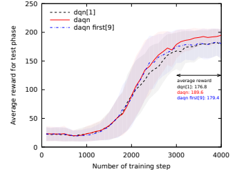
Fig. 3. Rewards for cart-pole game: that optimizer setting is only for auto-encoder (ae); the optimizer of dqn is same as dqn method.
