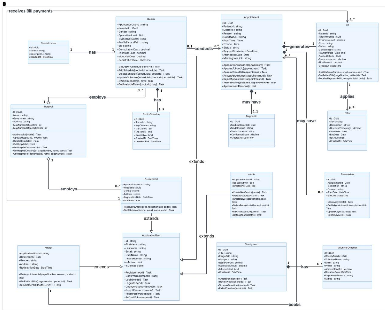
Figure 17.1 – Class Diagram
