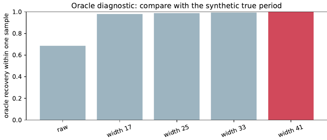
Figure 4: Output 2.2: oracle period recovery.
