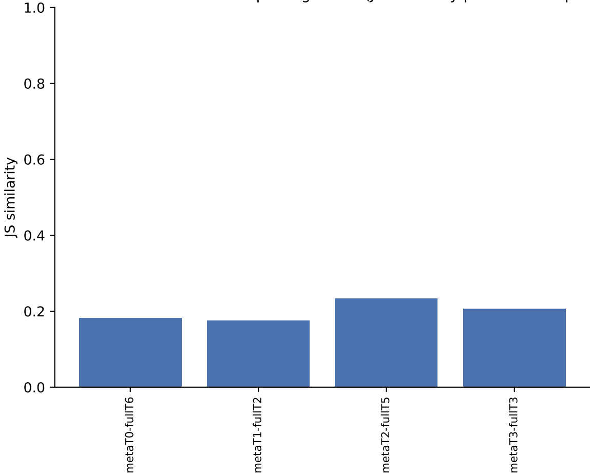
C1: Metadata vs. full-text topic-alignment (JS similarity per matched pair)
