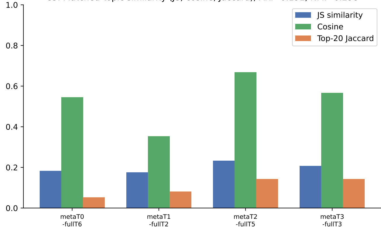
C3: Matched-topic similarity (JS, cosine, Jaccard); ARI=0.191, NMI=0.298
