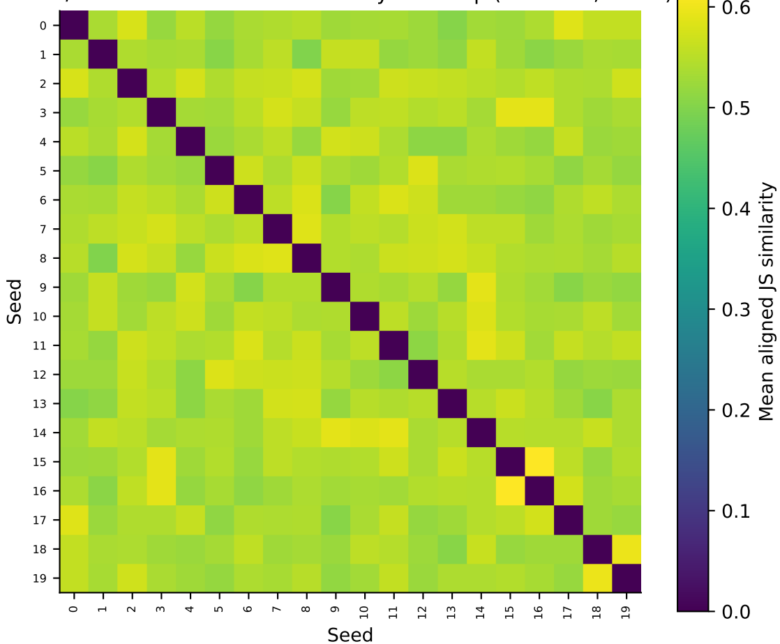
F10/F8: fulltext k=8 seed-similarity heatmap (20 seeds, N=66)
