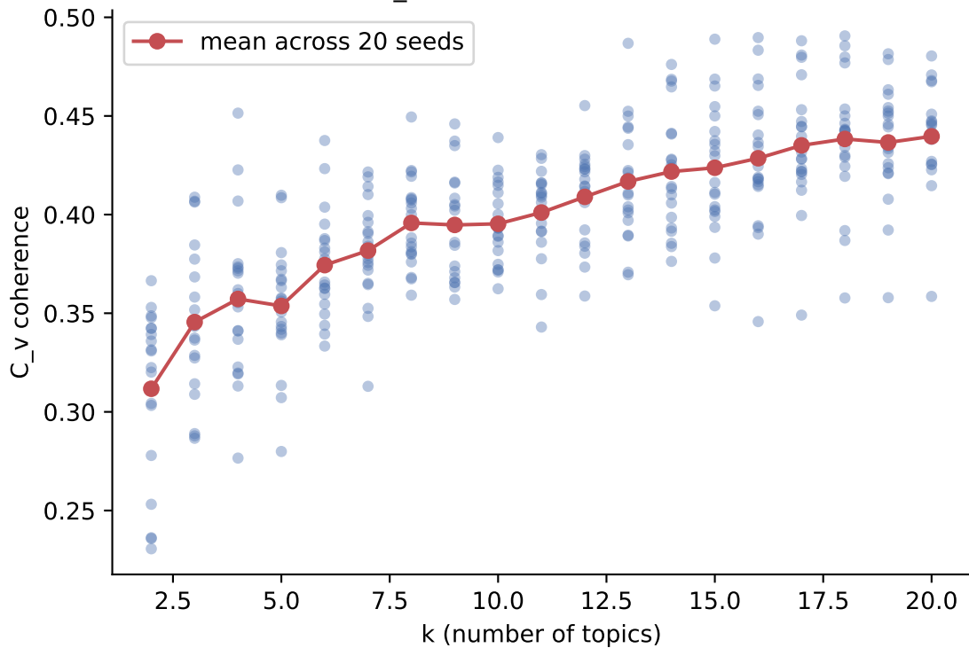
F1: fulltext C_v vs k (N=66, k=2-20, 20 seeds/k)
