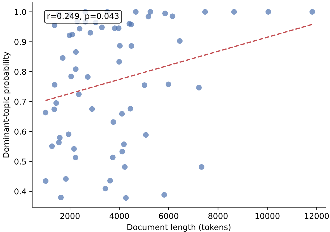
F20: Document length vs. topic-assignment confidence (N=66)
