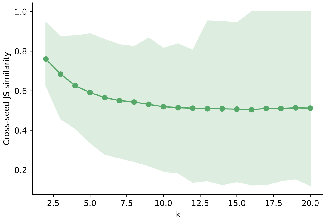
F3: fulltext cross-seed stability vs k (N=66, 20 seeds/k)
