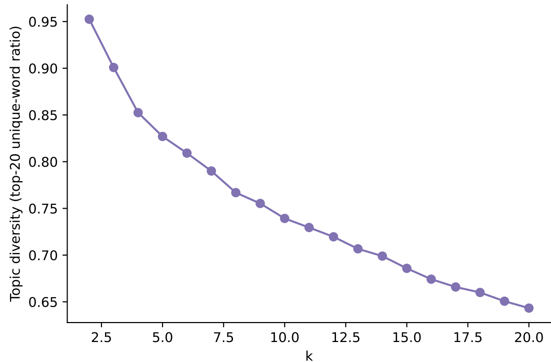
F4: fulltext topic diversity vs k (N=66)
