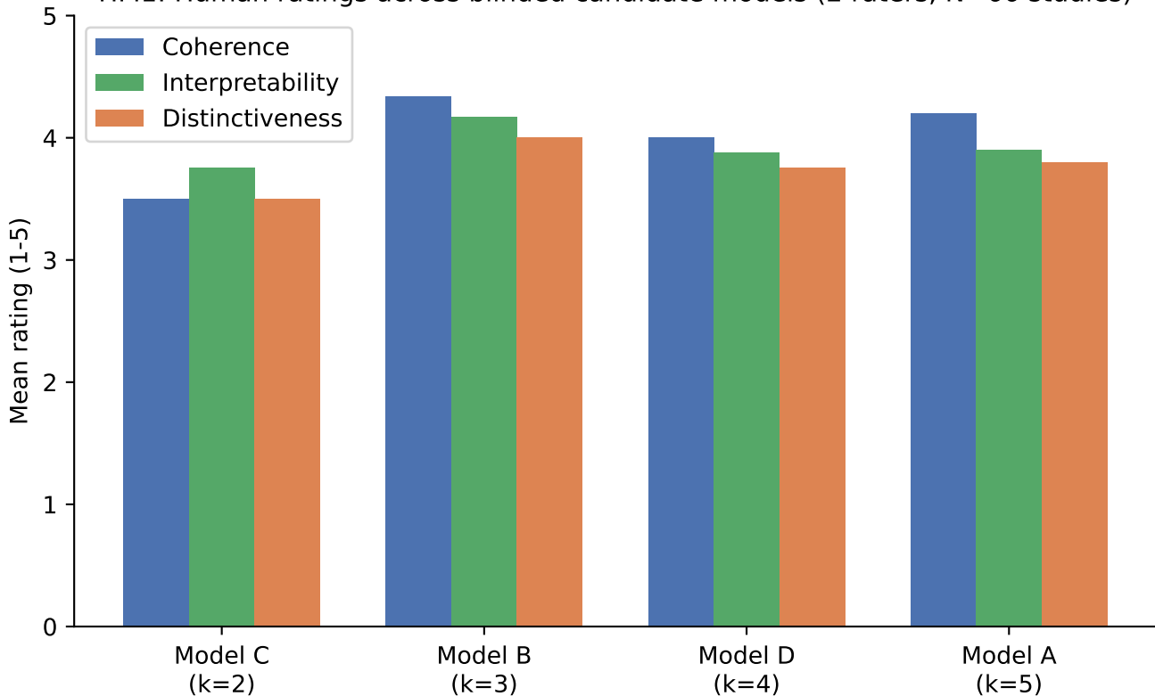
HM1: Human ratings across blinded candidate models (2 raters, N=66 studies)
