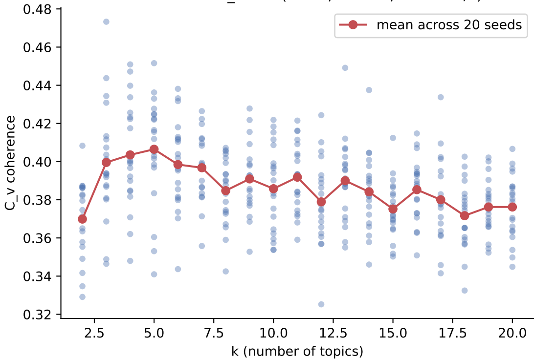
M1: metadata C_v vs k (N=66, k=2-20, 20 seeds/k)
