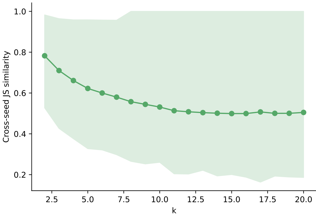
M3: metadata cross-seed stability vs k (N=66, 20 seeds/k)
