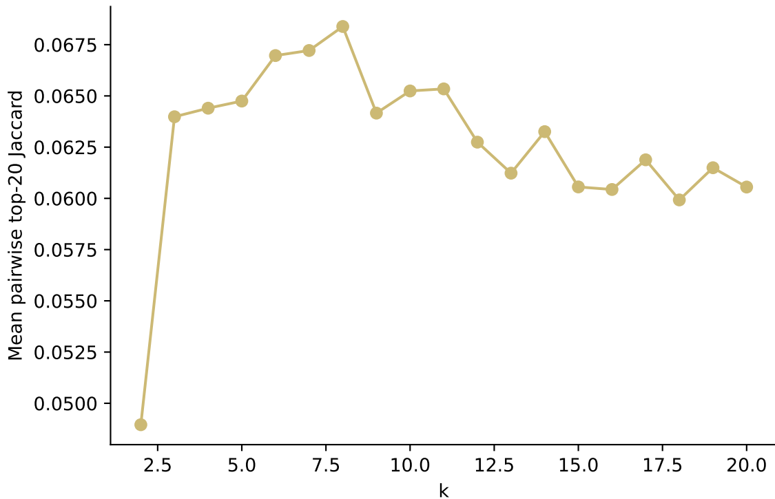
M5: metadata topic redundancy vs k (N=66)
