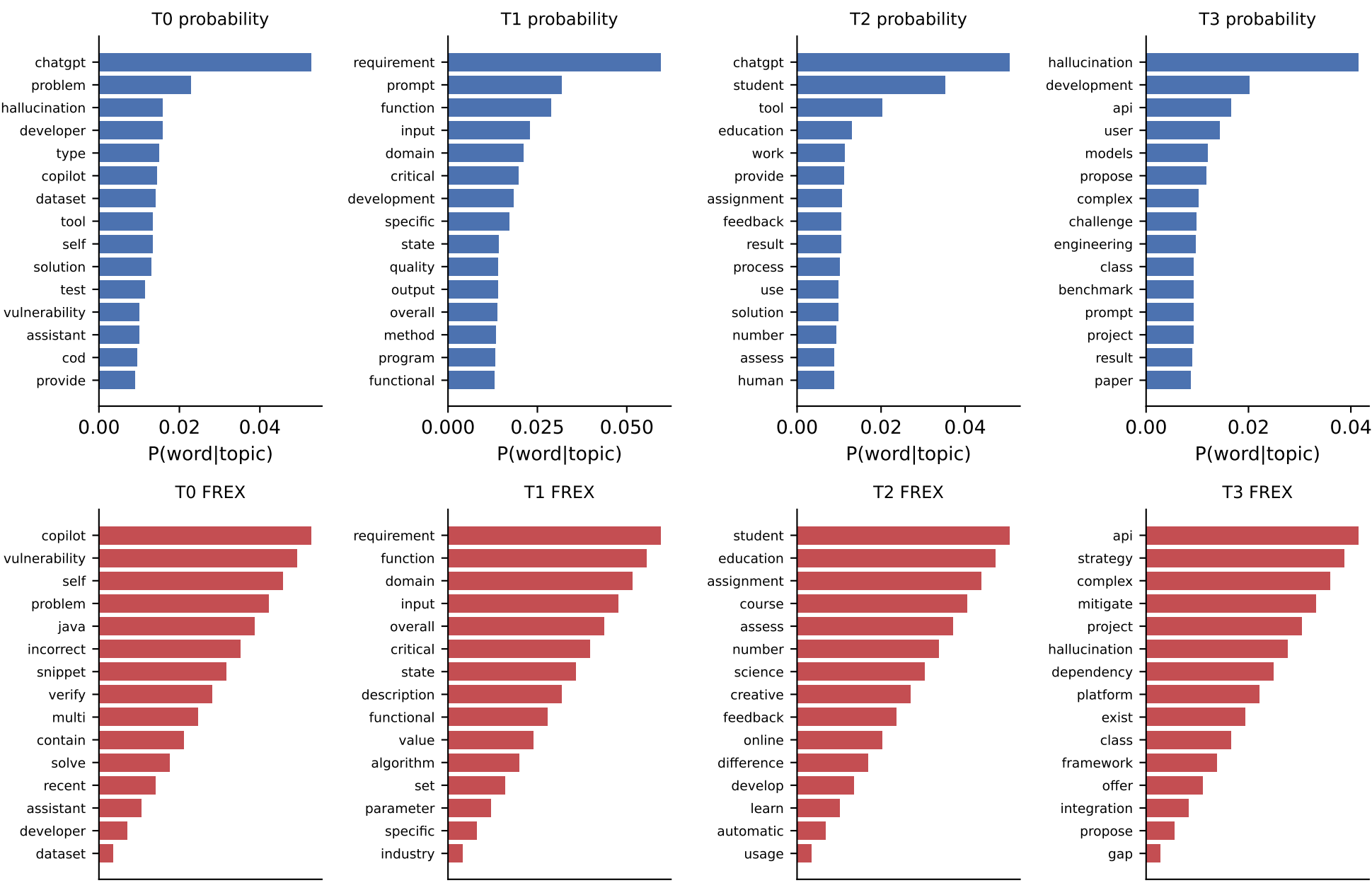
metadata final topics (k=4, seed=14): top-15 probability terms (top row) and top-15 FREX/exclusive terms (bottom row)
