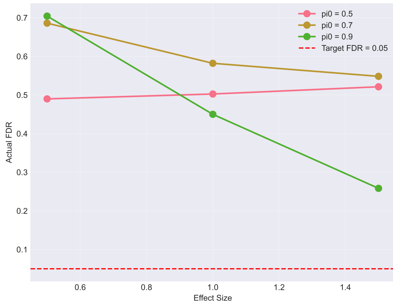
FDR Control Performance
