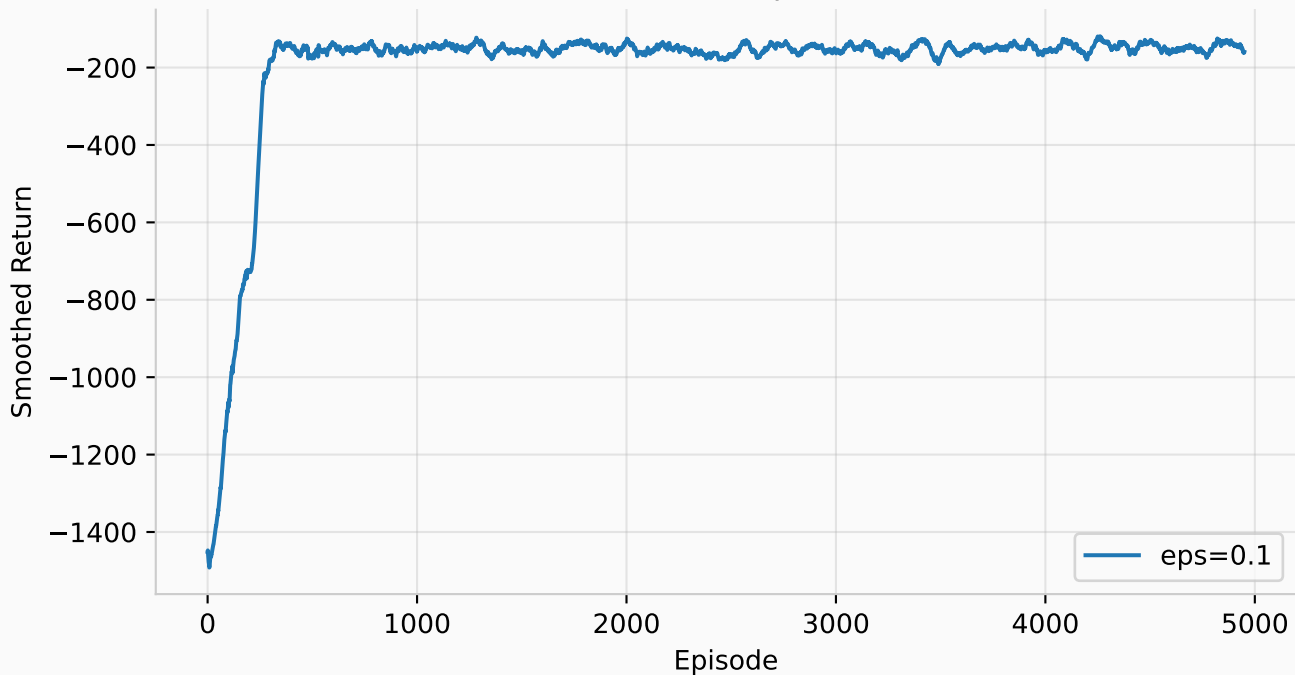
TD3 on Pendulum-v1 — exploration noise scale
