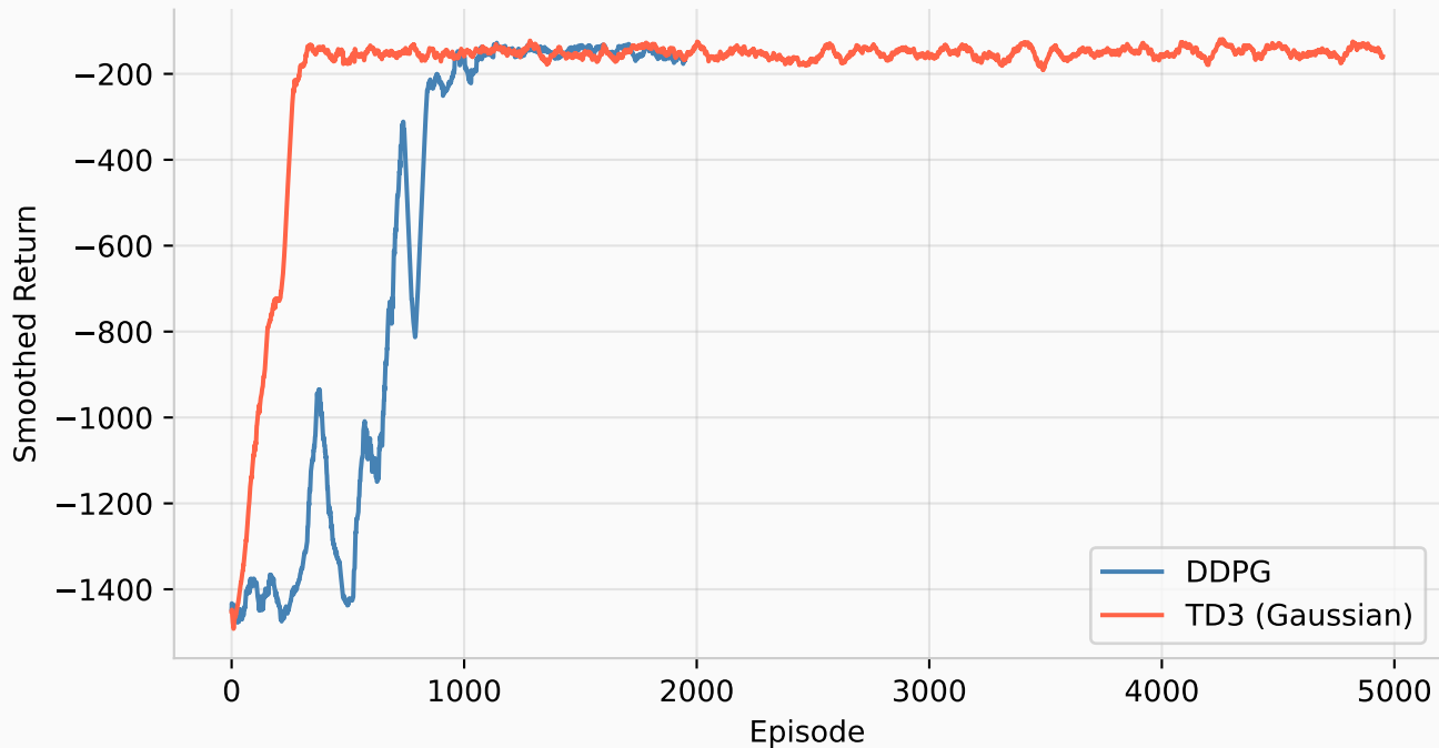
TD3 vs DDPG on Pendulum-v1
