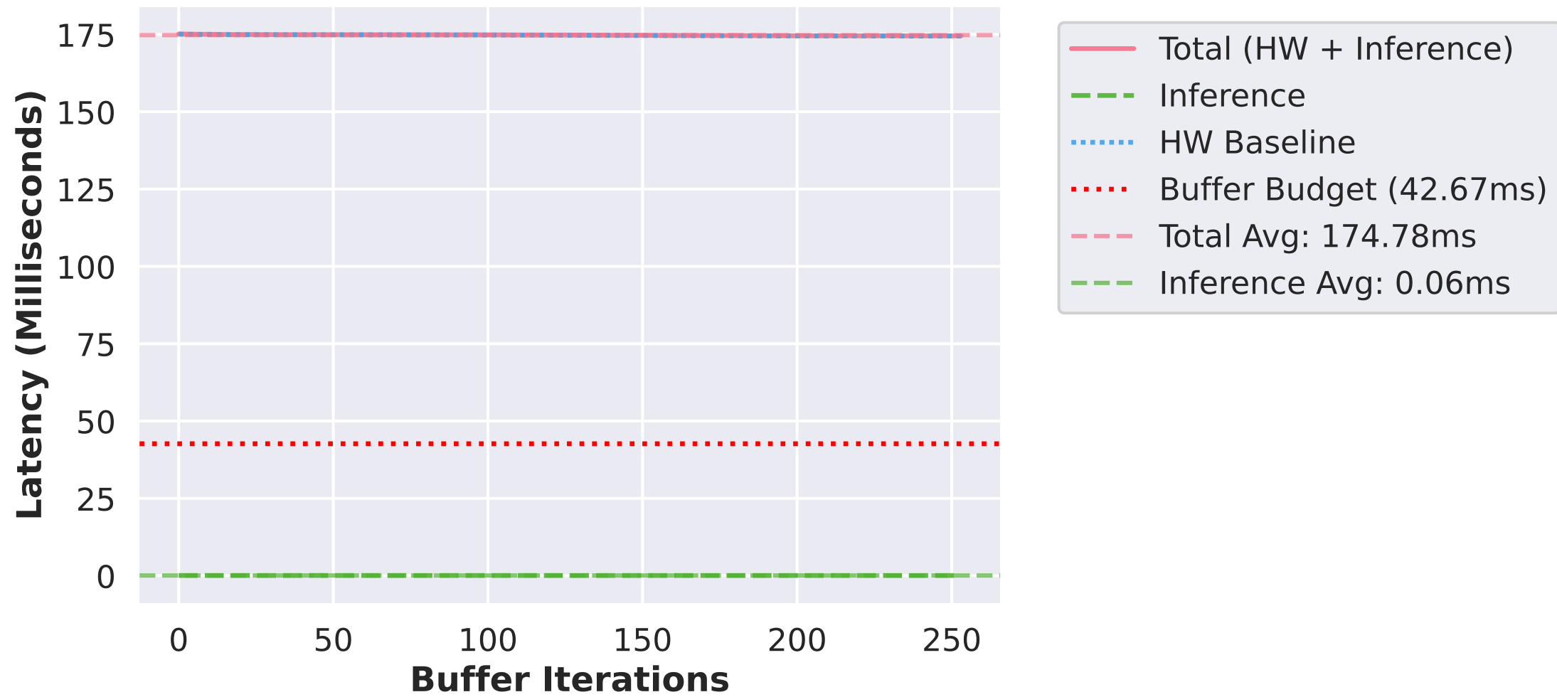
Real-Time Pitch Correction Latencies (Skipping First 20 Iterations)
