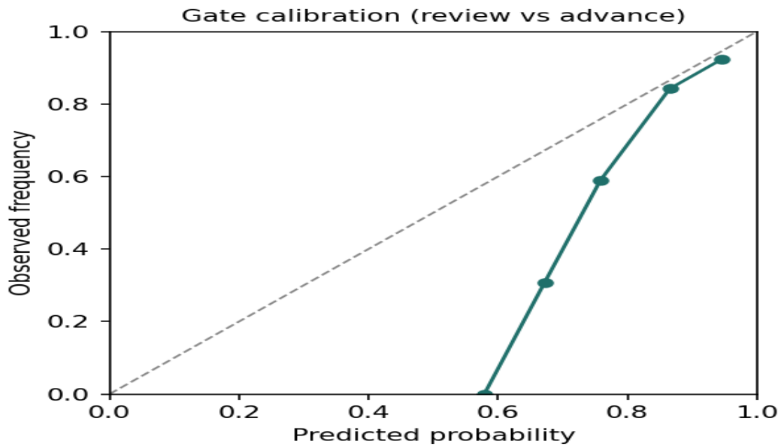
fig_gate_reliability.png
