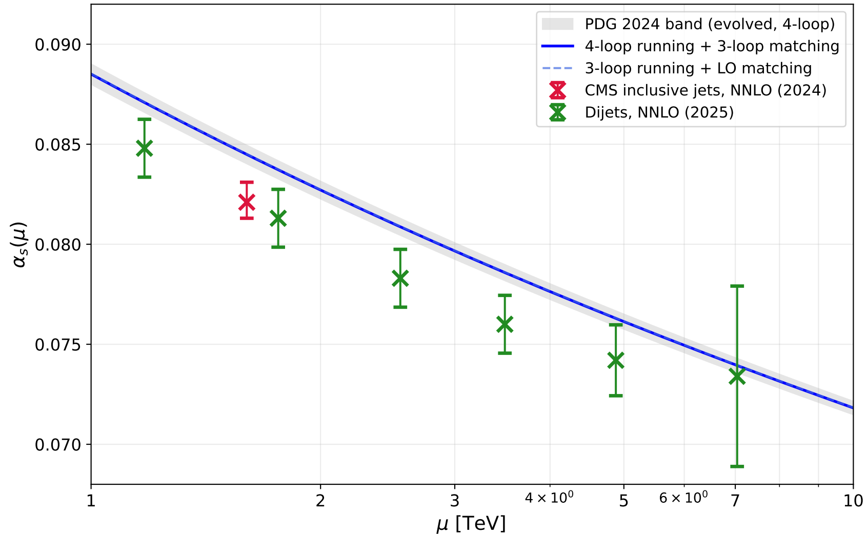
Running of \alpha_s in the TeV range
