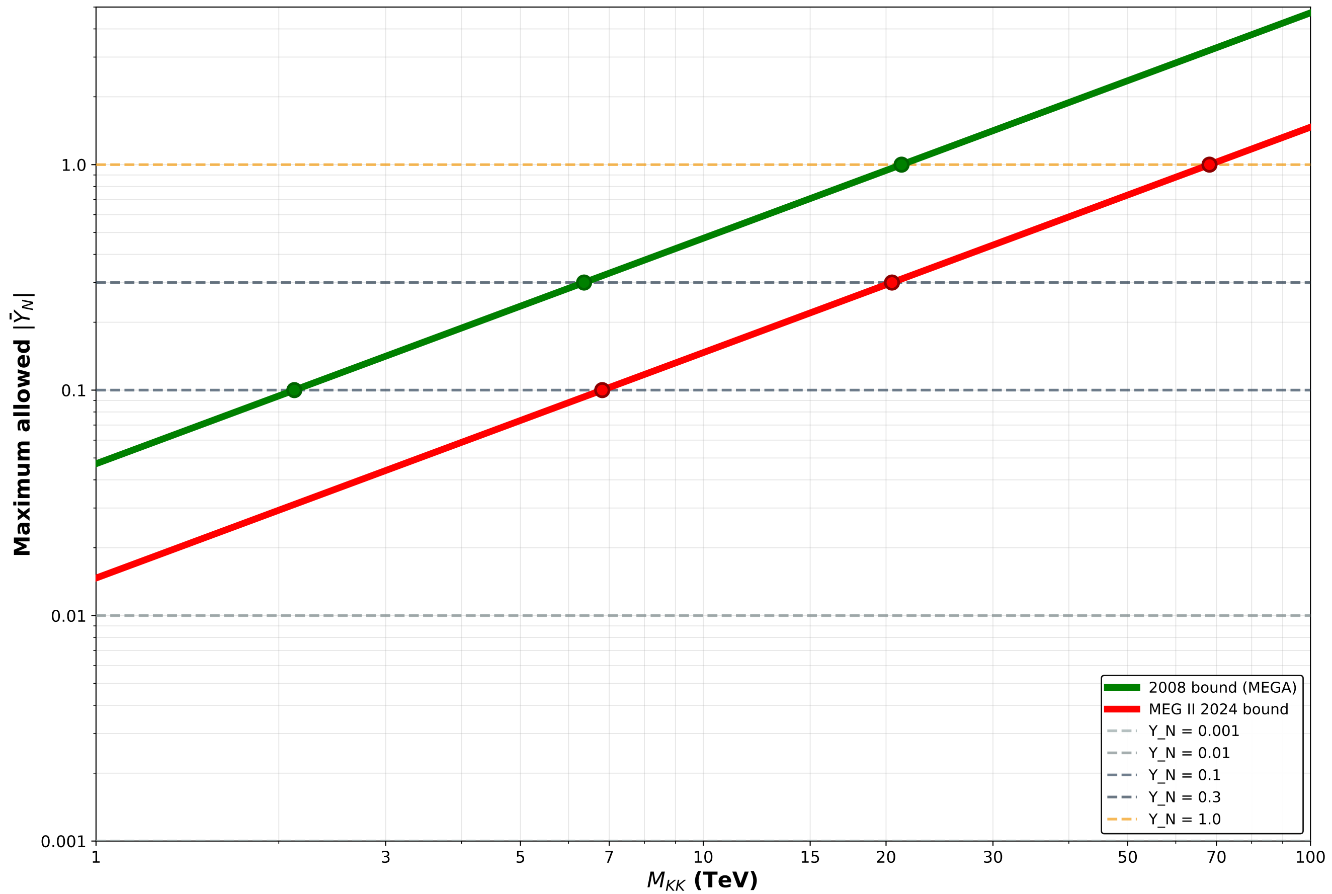
The Yukawa-M_KK Trade-off: What Y_N Can You Achieve at Each M_{KK} ?
