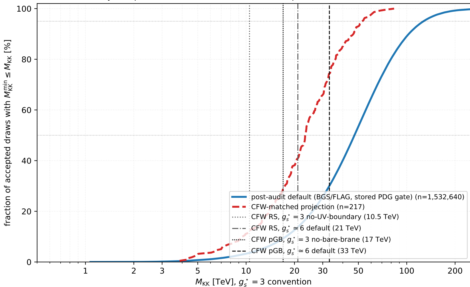
RS-anarchy comparison to Csaki--Falkowski--Weiler (post-audit vs convention-matched)
