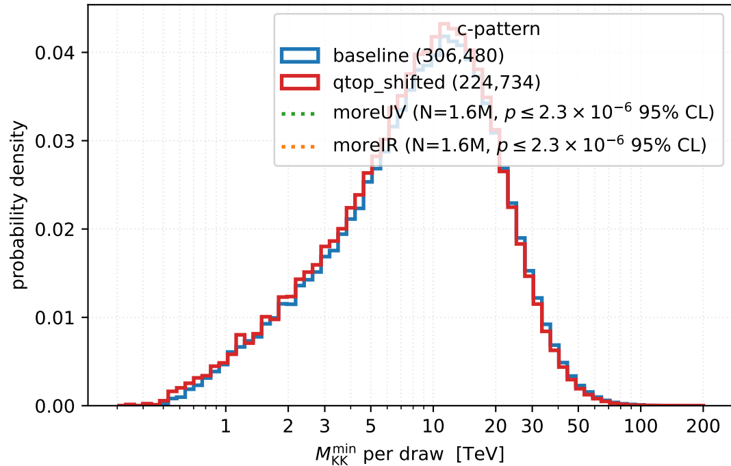
Per-draw M_{\text{KK}}^{\text{min}} vs c-value pattern
