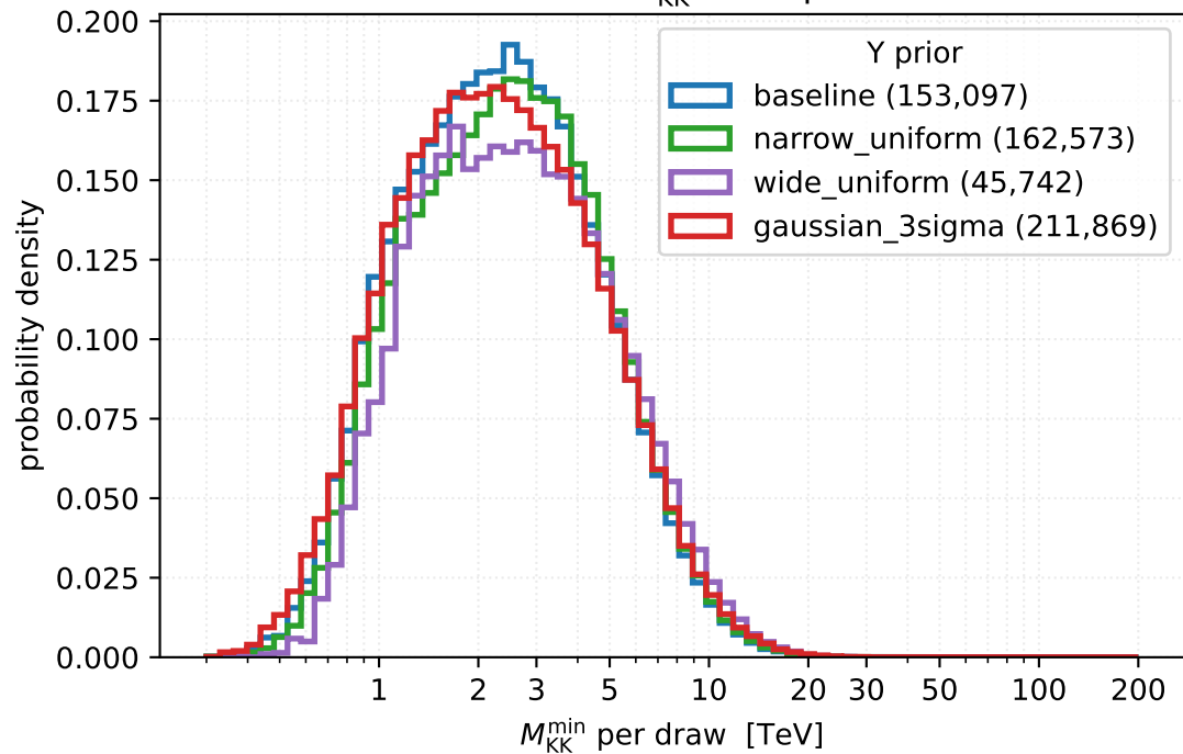
Per-draw M_{KK}^{\min} vs Y-prior
