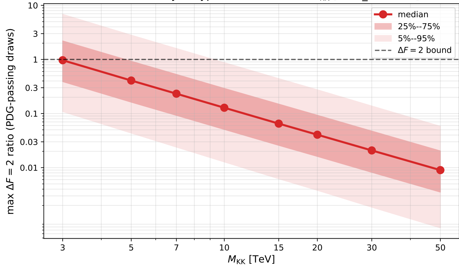
RS flavor anarchy --- typical FCNC ratio vs M_{\text{KK}} [runA_8Mdraws]
