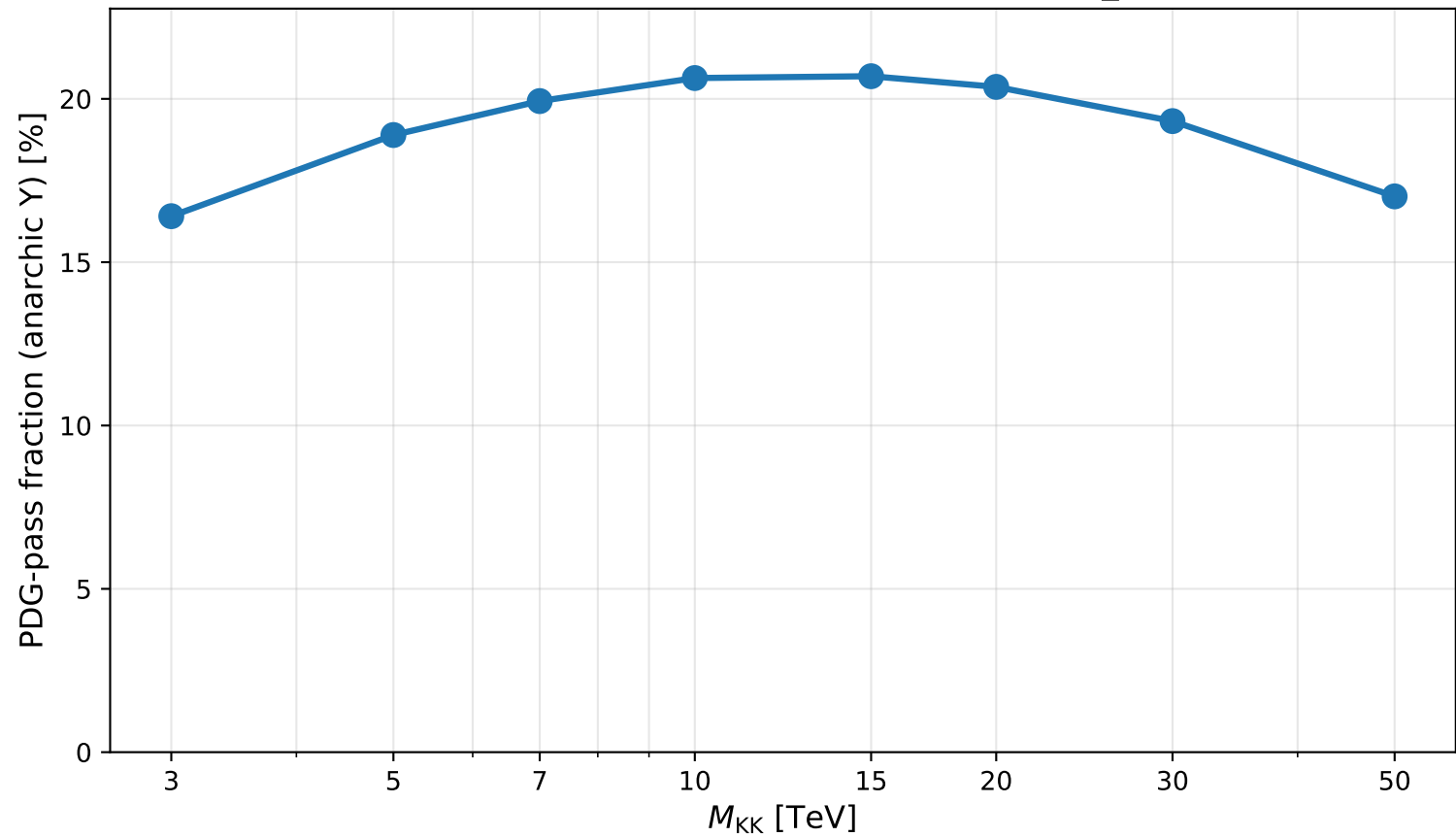
RS flavor anarchy --- PDG-pass rate vs M_{KK} [runA_8Mdraws]
