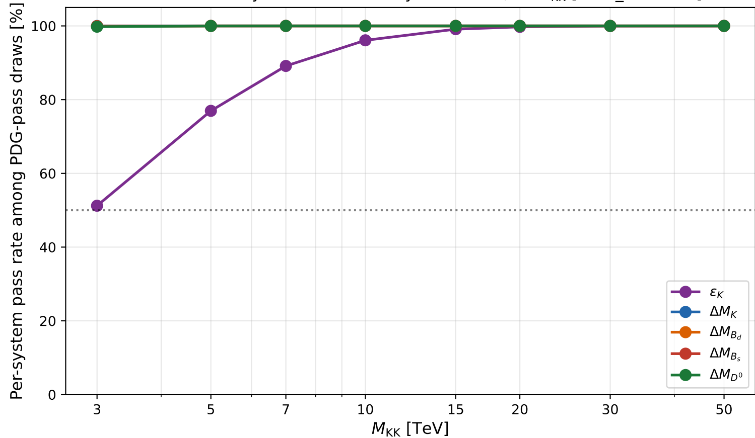
RS flavor anarchy --- which \Delta F = 2 system binds, vs M_{KK} [runA_8Mdraws]
