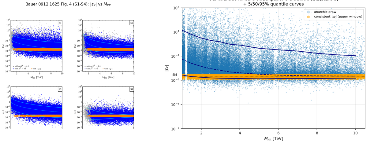
Figure 4: Anarchy |\varepsilon_K| vs. M_{KK} : paper (left) vs. ours (right), with 5/50/95% quantile curves. Paper scatters anarchic Yukawas; we reproduce the fat cloud in anarchic-forward mode.
