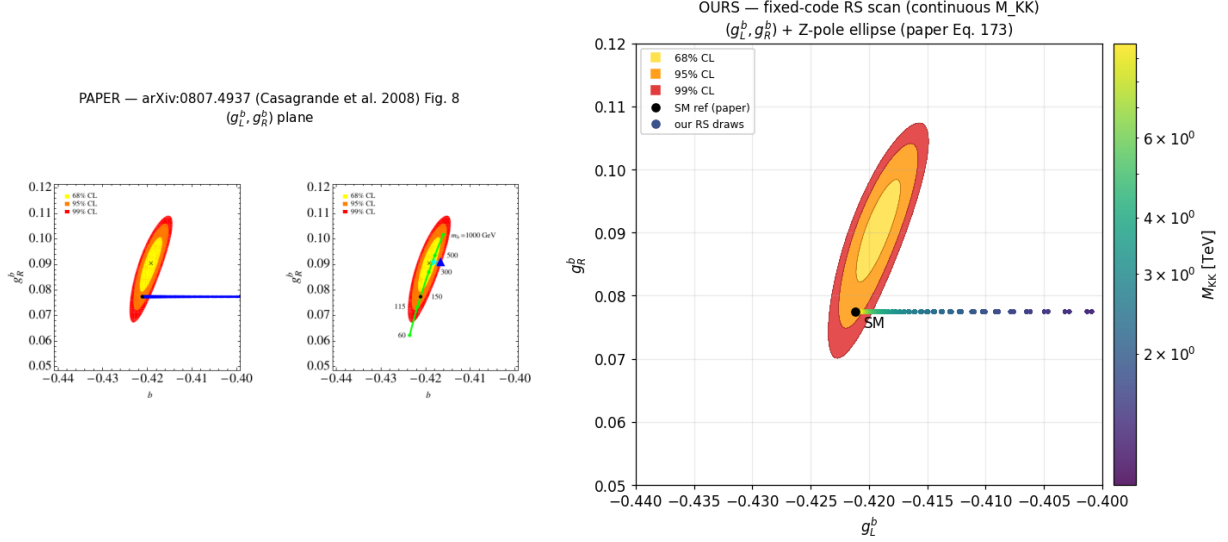
Figure 3: The (g_L^b, g_R^b) plane: paper (left) vs. ours (right), with the Z -pole CL ellipses and the SM point.
