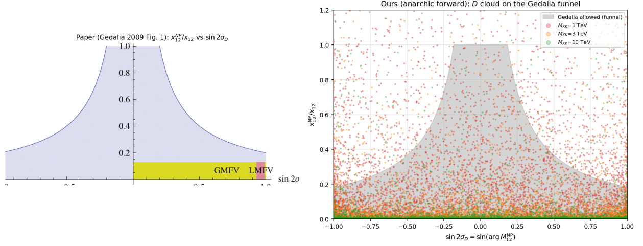
Figure 8: The allowed “funnel” in (x_{12}^{\text{NP}}/x, \sin 2\sigma_D) : paper (left) vs. ours (right). Our cloud sinks into the allowed funnel as M_{KK} rises.
