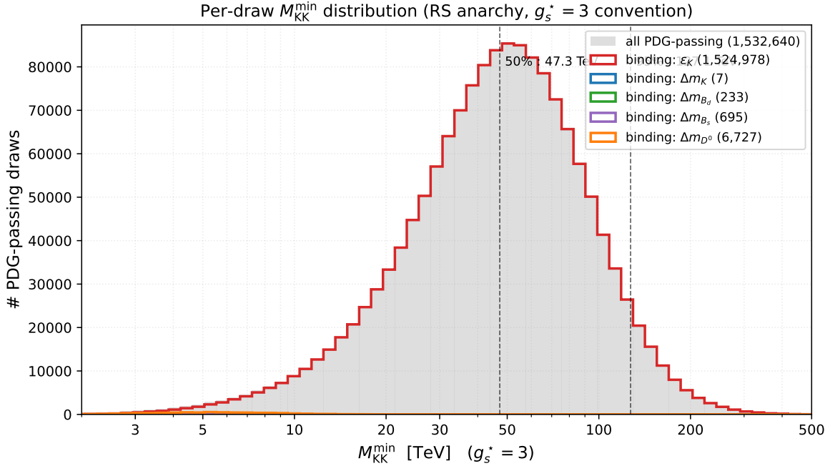
Figure 2: Per-draw M_{\text{KK}}^{\text{min}} histogram for the RS-anarchy ensemble, restricted to draws that pass the factor-of-three PDG mass and CKM match (1,532,640 draws total from the 8M-draw RUNA reference scan, pooled across all eight M_{\text{KK}} tiles). The x-axis is in the g_s^* = 3 convention, the headline convention used throughout this note. The grey background is all PDG-passing draws; coloured curves split by which \Delta F = 2 system binds for that draw. The vast majority are \varepsilon_K -bound; the \Delta m_K, \Delta m_{B_d}, \Delta m_{B_s}, \Delta m_{D^0} contributions live in the low- M_{\text{KK}}^{\text{min}} tail. Vertical dashed lines mark the 50%- and 95%-acceptance crossings.
