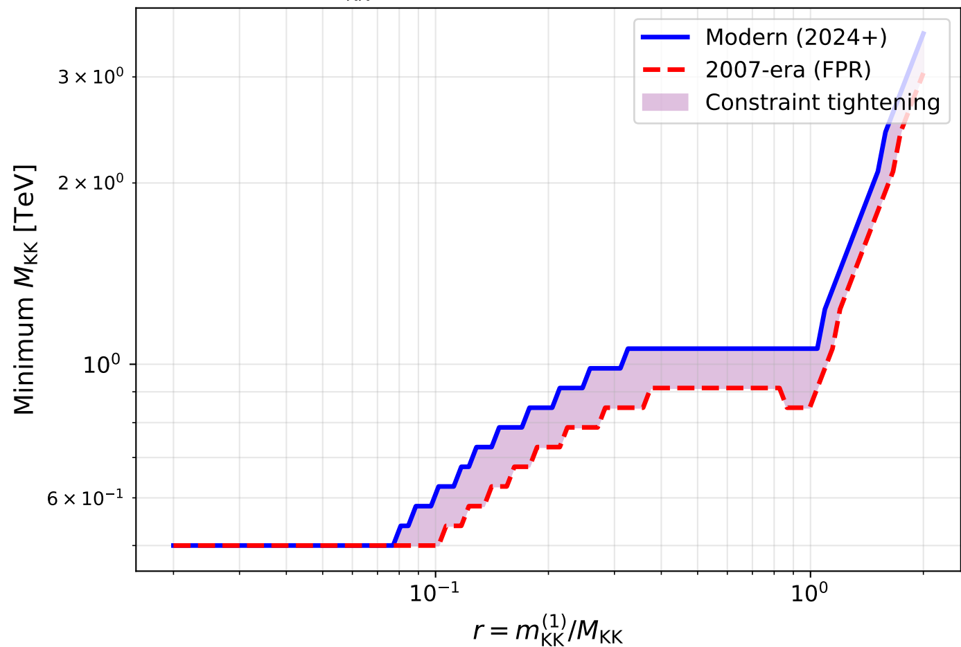
M_{\text{KK}} Lower Bound: 2007 vs Modern
