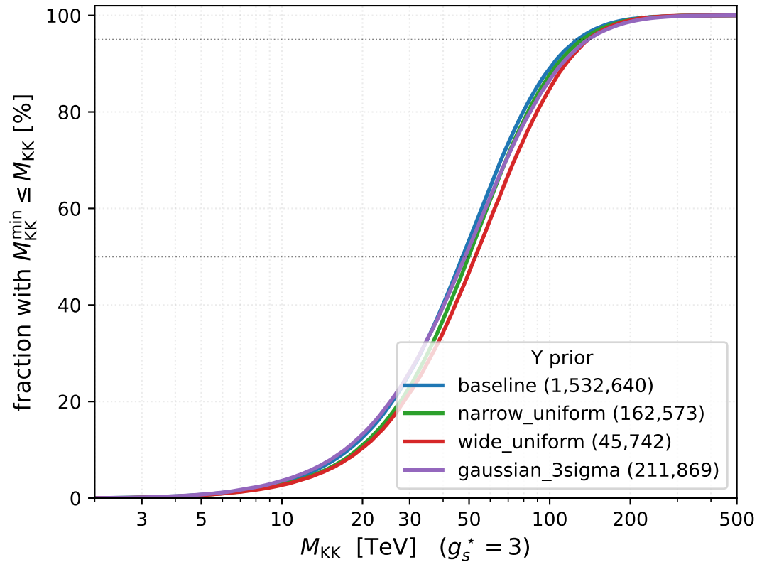
Cumulative distribution ( g_s^* = 3 )
