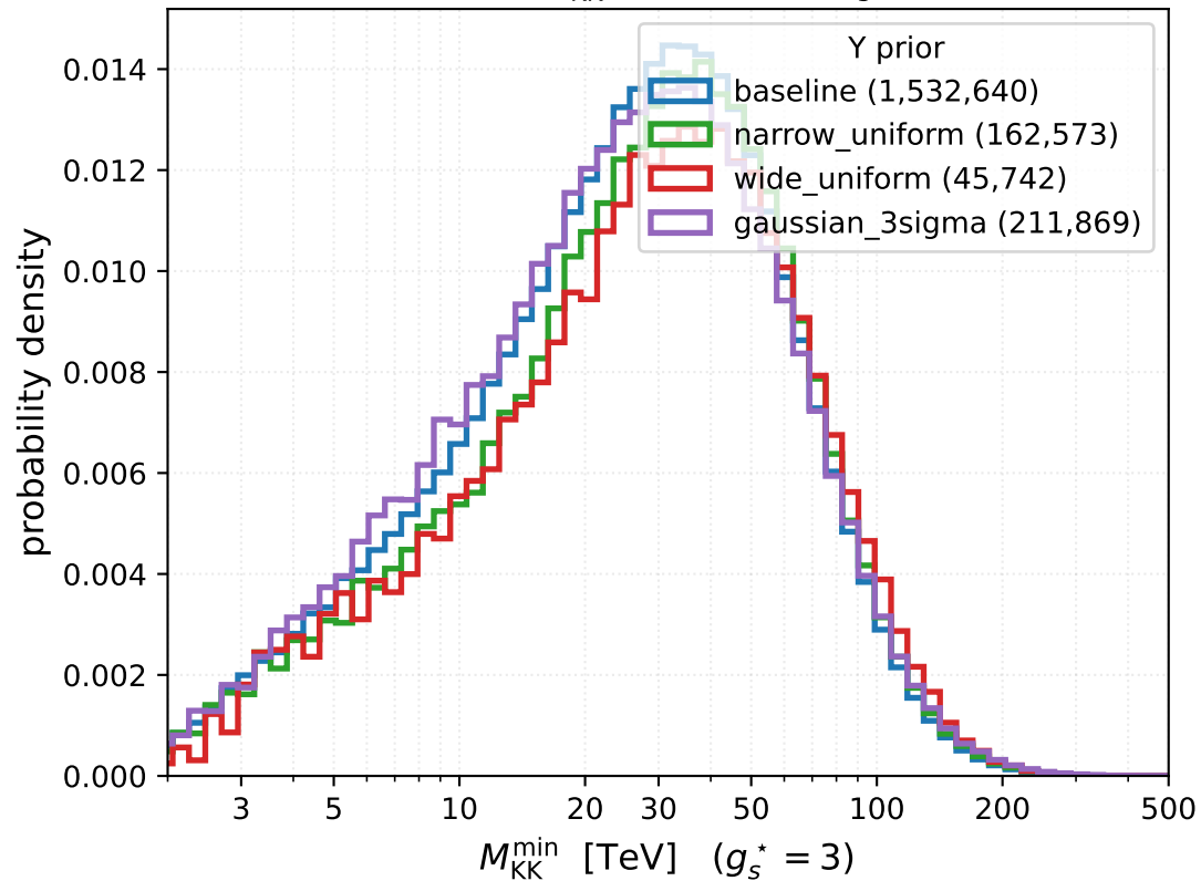
Per-draw M_{\text{KK}}^{\text{min}} vs Y-prior ( g_s^* = 3 )
