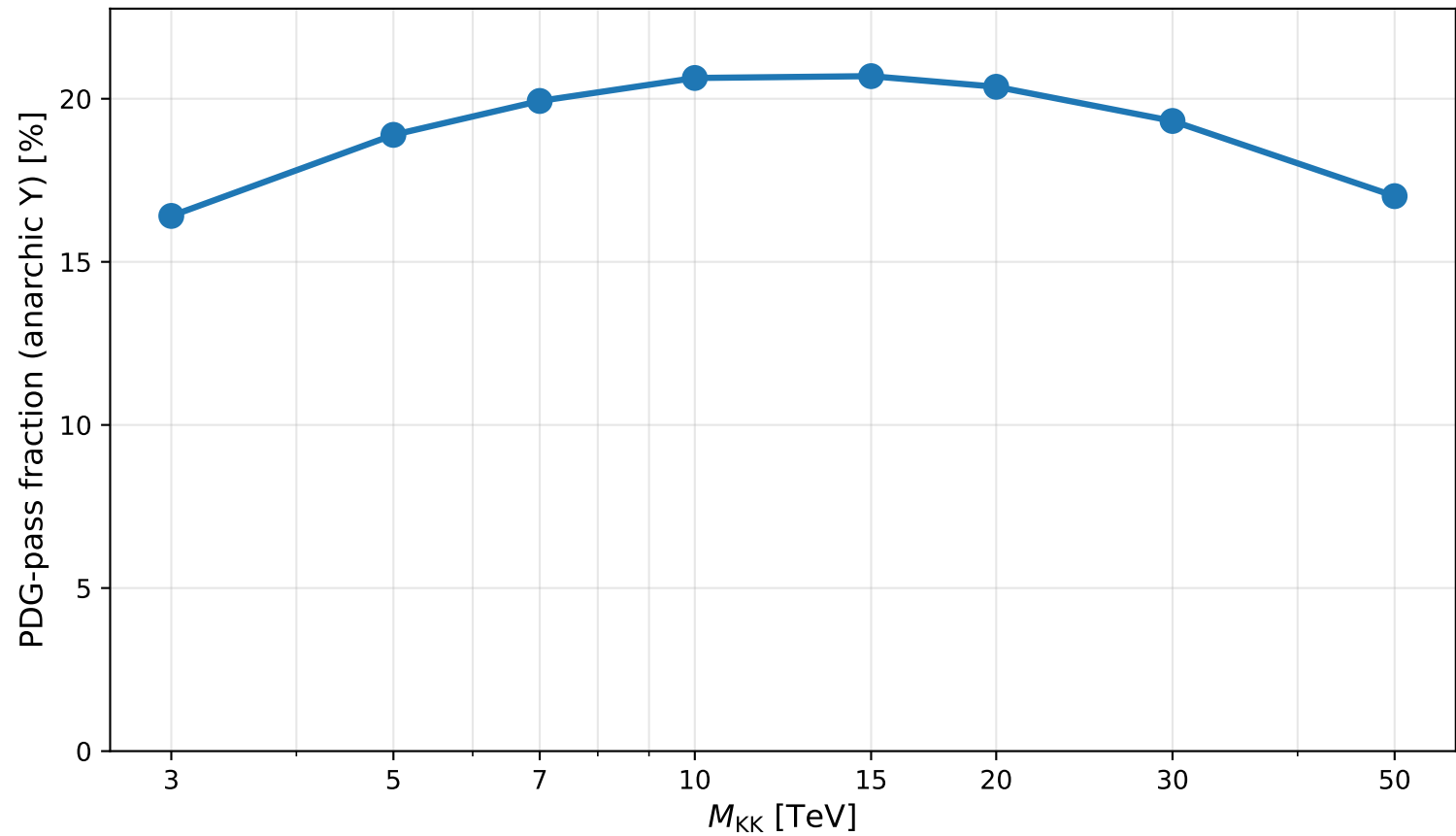
RS flavor anarchy --- PDG-pass rate vs M_{\text{KK}}
