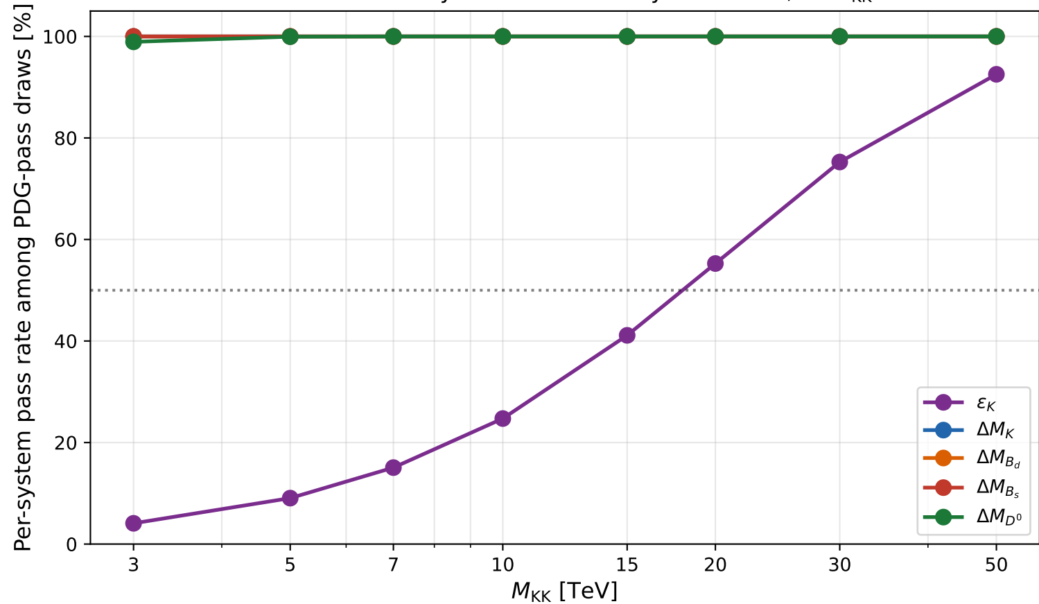
RS flavor anarchy --- which \Delta F = 2 system binds, vs M_{KK}
