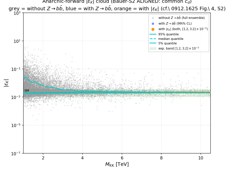
Figure 6: Alignment endpoint (Bauer-S2, common right-handed down c_d via a U(3) degeneracy): the cloud stays fat but gains \varepsilon_K -consistent points, dropping the floor toward \sim 1.8 TeV — a cure that imposes structure rather than predicting it.
