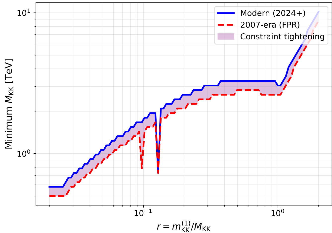
M_{\text{KK}} Lower Bound: 2007 vs Modern
