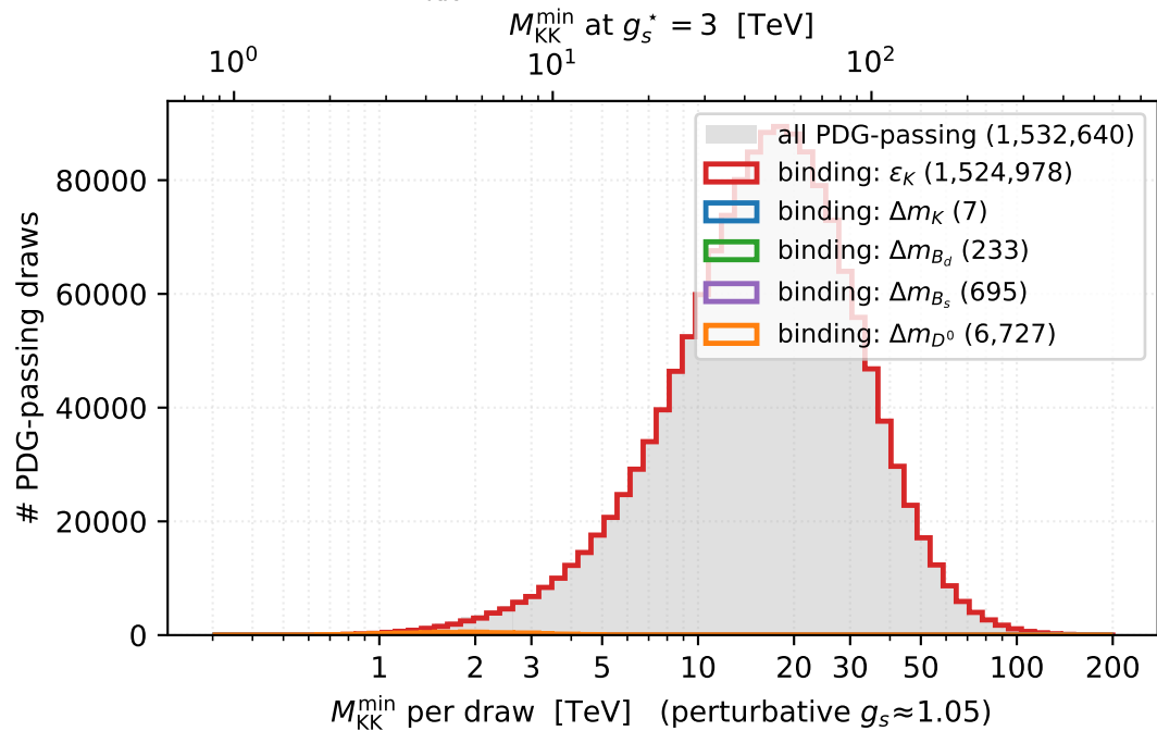
Per-draw M_{KK}^{\min} distribution, by binding observable
