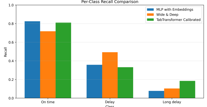
Fig. 6. Per-class recall comparison across the main models.
