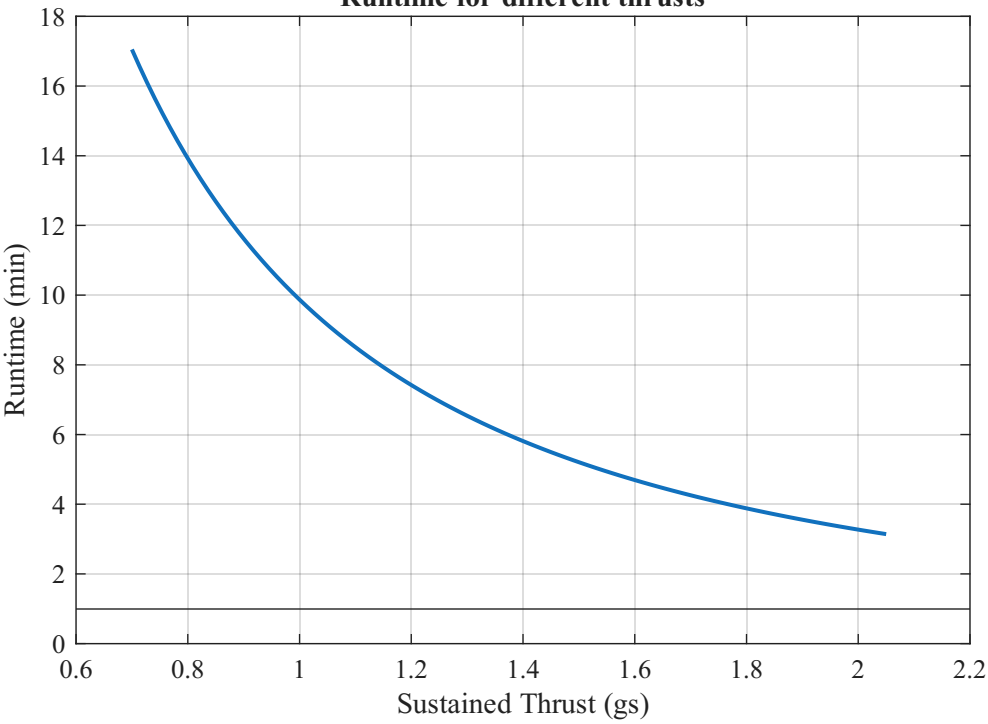
Runtime for different thrusts
