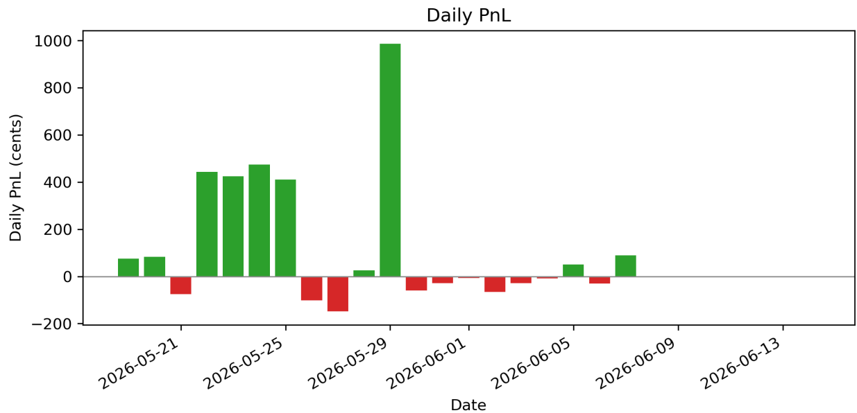
Figure 11: Daily net PnL across the MCP simulation window.
