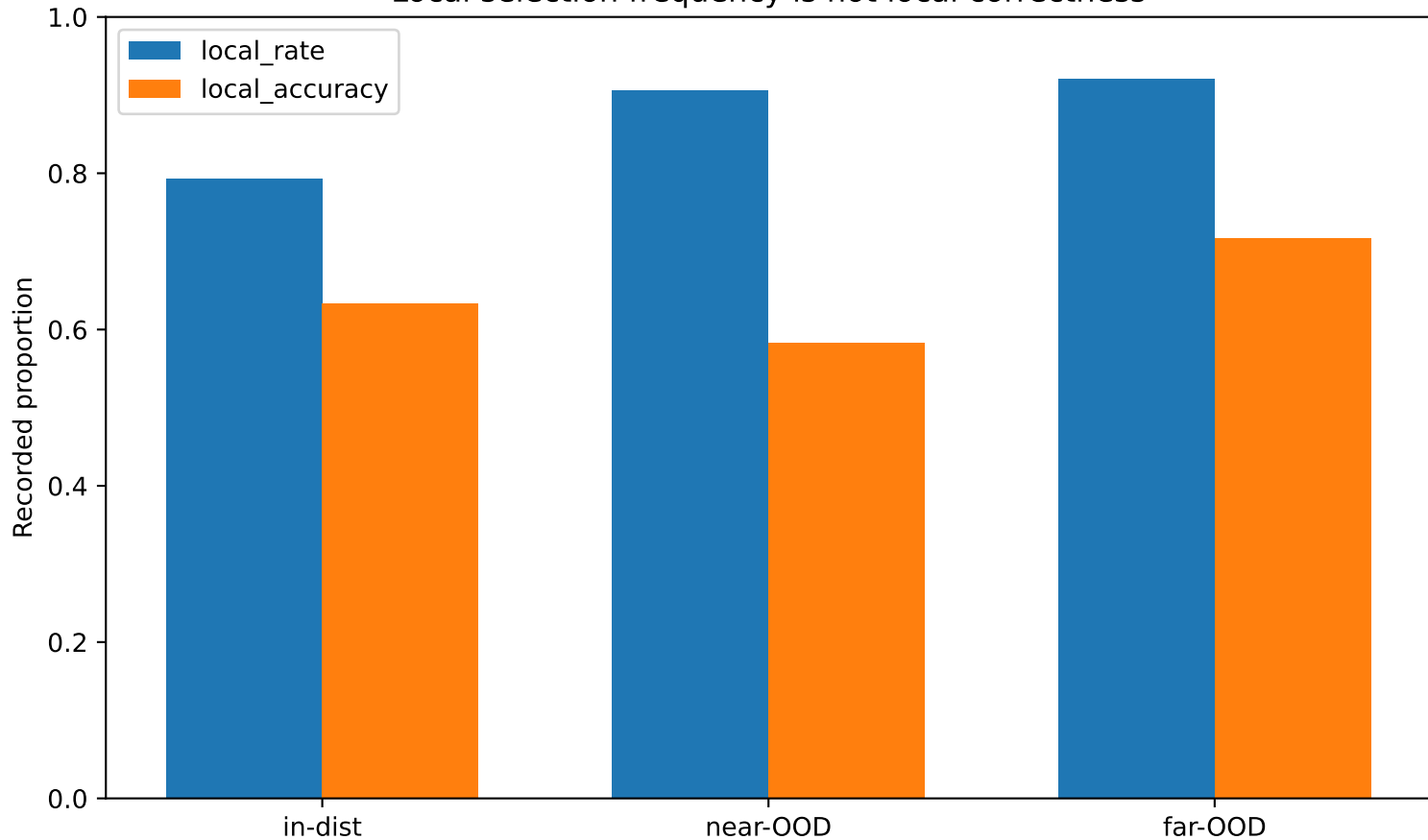
Local selection frequency is not local correctness
