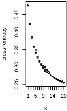
sorghum_la
