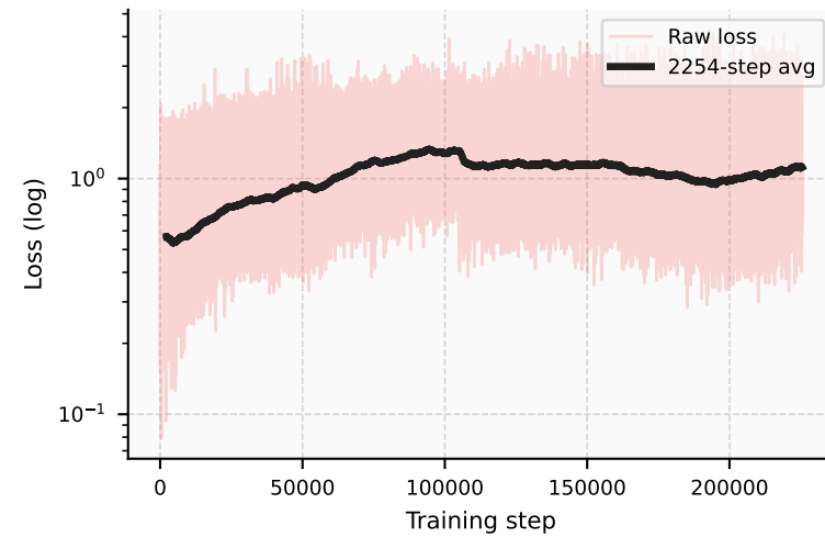
Training Loss (Huber)
