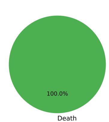
Outcome Distribution
