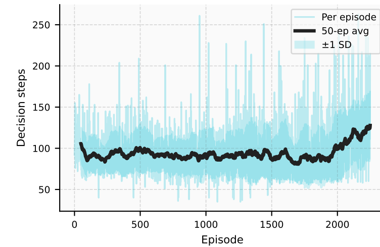
Episode Length
