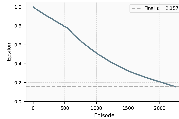
Exploration Rate ( \epsilon )
