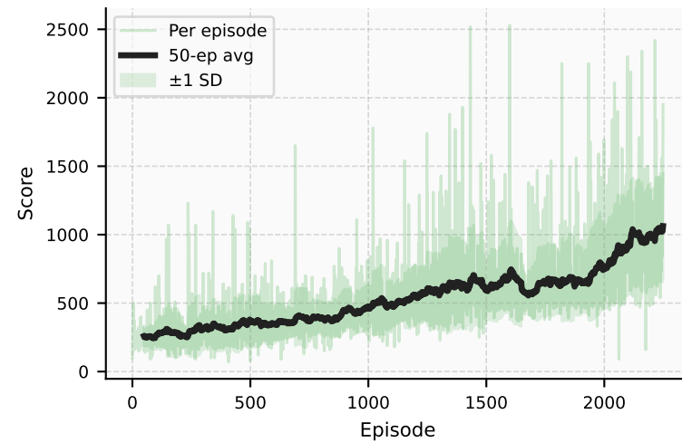
Game Score
