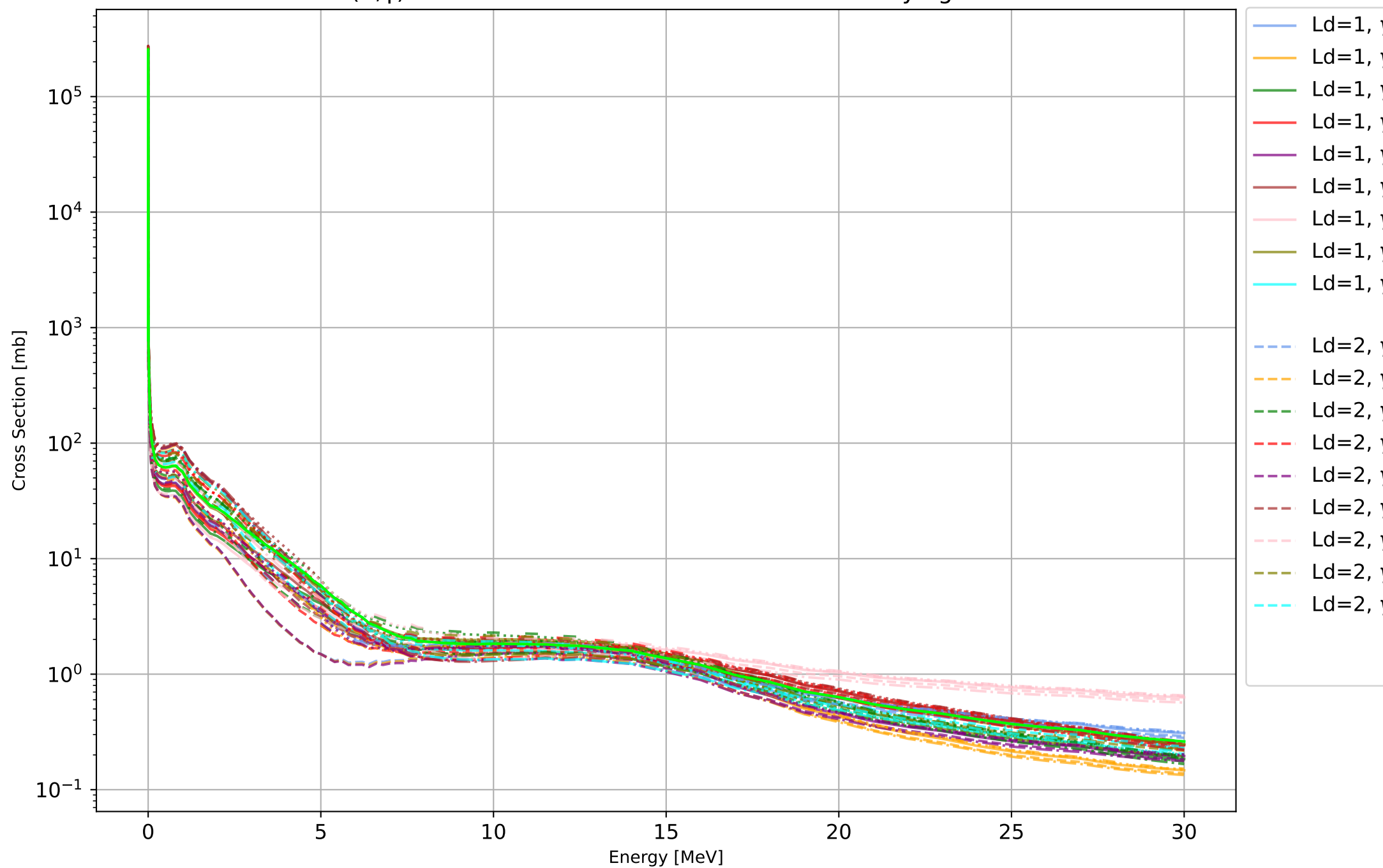
^{119}\text{Sn}(n,\gamma)^{120}\text{Sn} Cross Sections from TALYS with Varying Models
