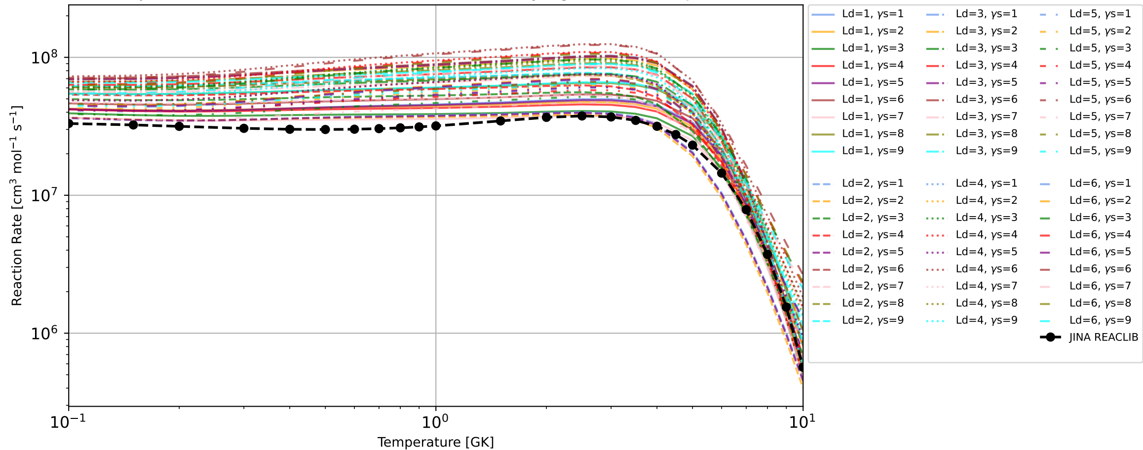
^{119}\text{Sn}(n,\gamma)^{120}\text{Sn} reaction rates from TALYS with Varying Models and JINA REACLIB
