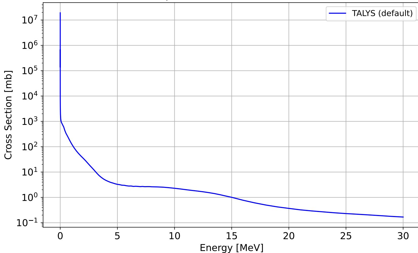
^{191}\text{Os}(n,\gamma)^{192}\text{Os} cross section from TALYS
