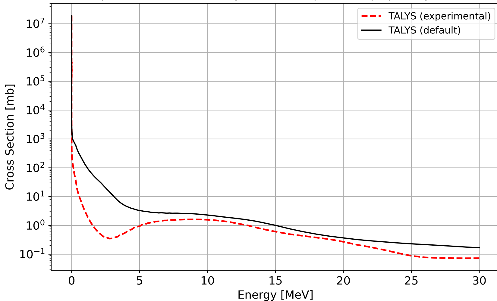
^{191}\text{Os}(n,\gamma)^{192}\text{Os} Cross Sections Using Default and Experimental \gamma -ray Strength Functions
