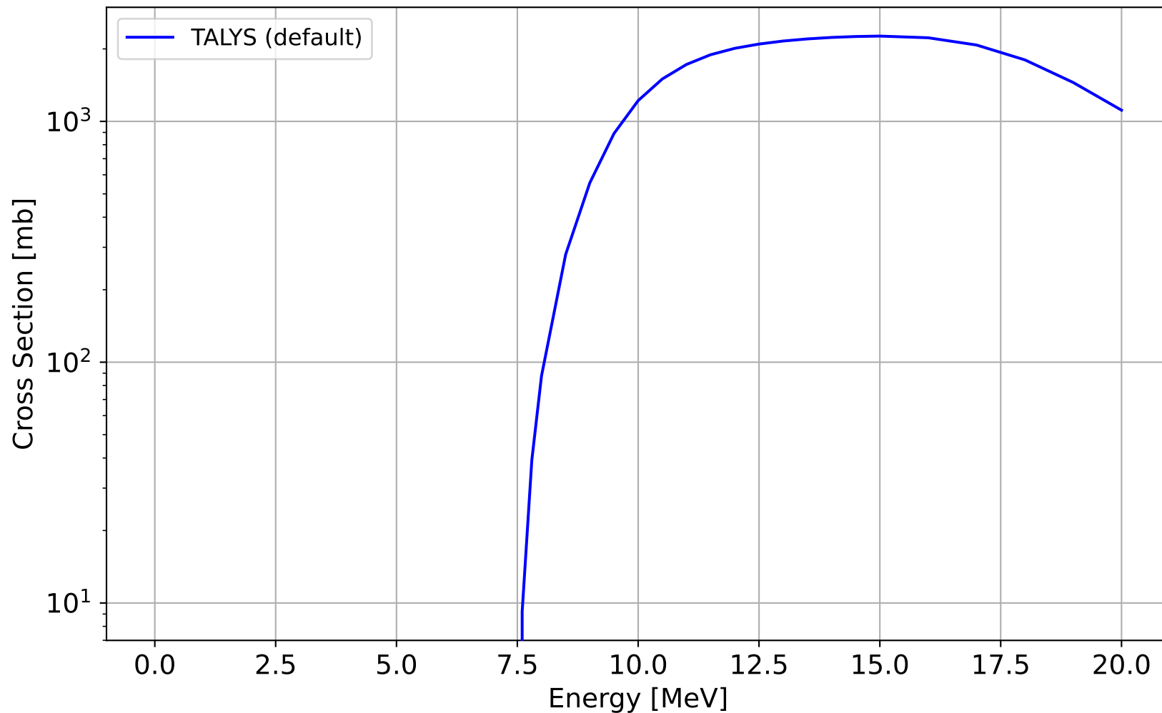
^{208}\text{Pb}(n,2n)^{207}\text{Pb} cross section from TALYS
