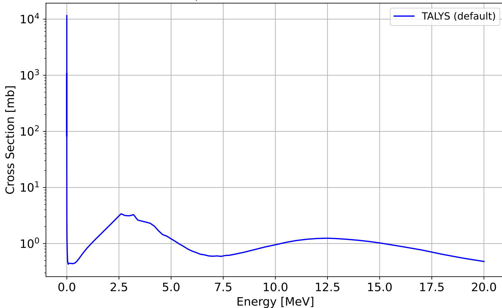
^{208}\text{Pb}(n,\gamma)^{209}\text{Pb} cross section from TALYS
