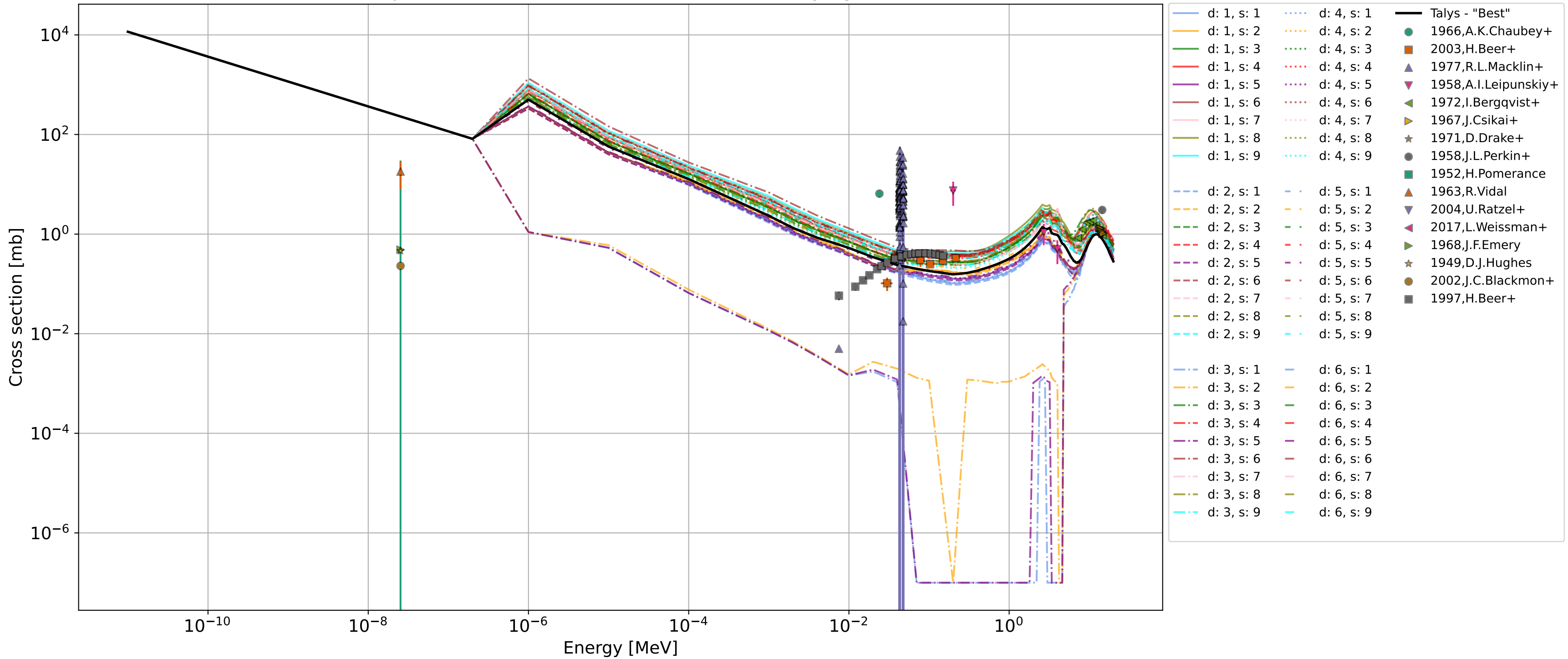
^{208}\text{Pb}(n,\gamma)^{209}\text{Pb} Cross Sections from TALYS with Varying Models
